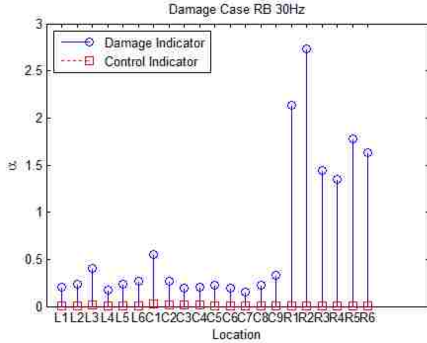
Figure 3.32 Lab Damage Scenario RB with 30Hz Input
