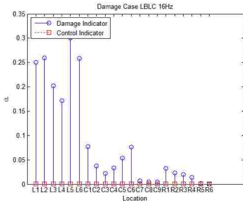
Figure 3.6 Simulation Damage Scenario LBLC with 16Hz Input
