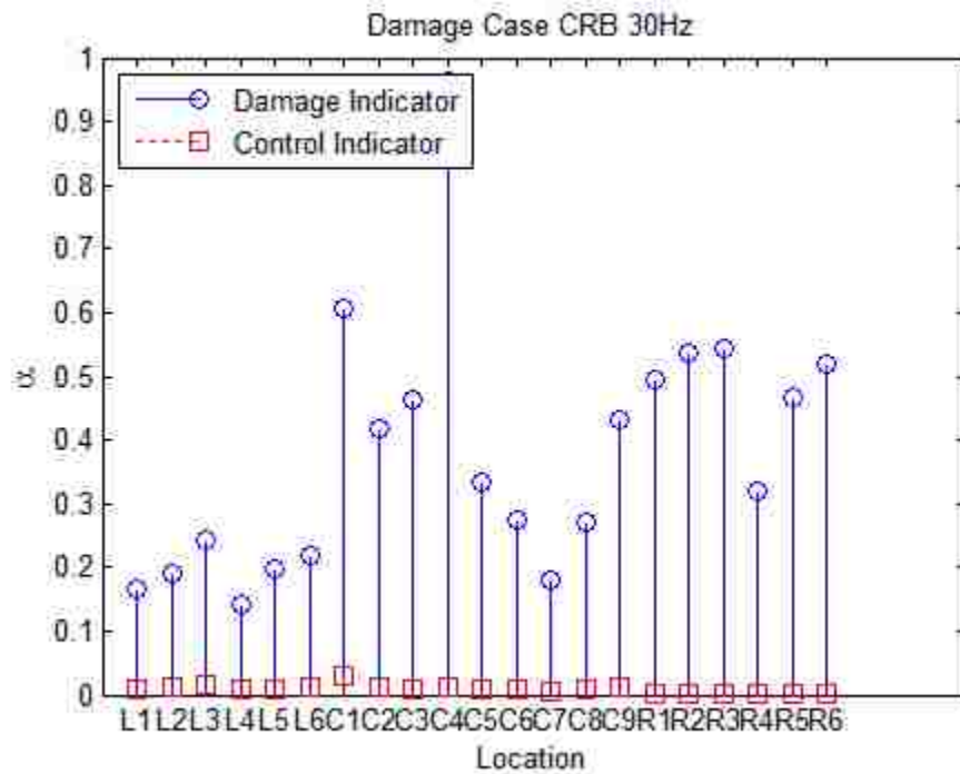
Figure 3.29 Lab Damage Scenario CRB with 30Hz Input
