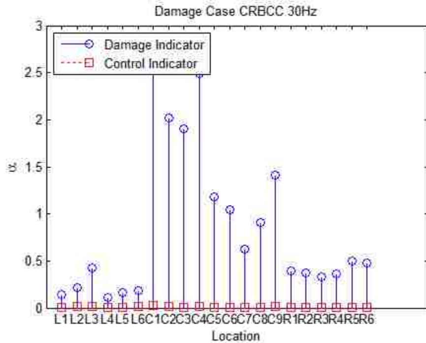
Figure 3.31 Lab Damage Scenario CRBCC with 30Hz Input
