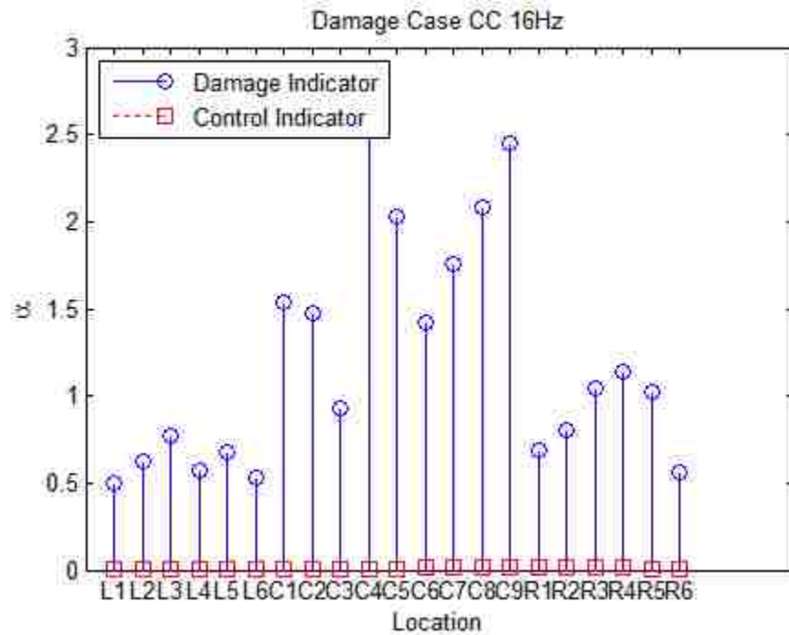
Figure 4.22 Lab Damage Scenario CC with 16Hz
