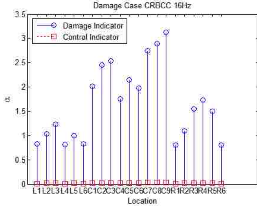
Figure 4.23 Lab Damage Scenario CRBCC with 16Hz
