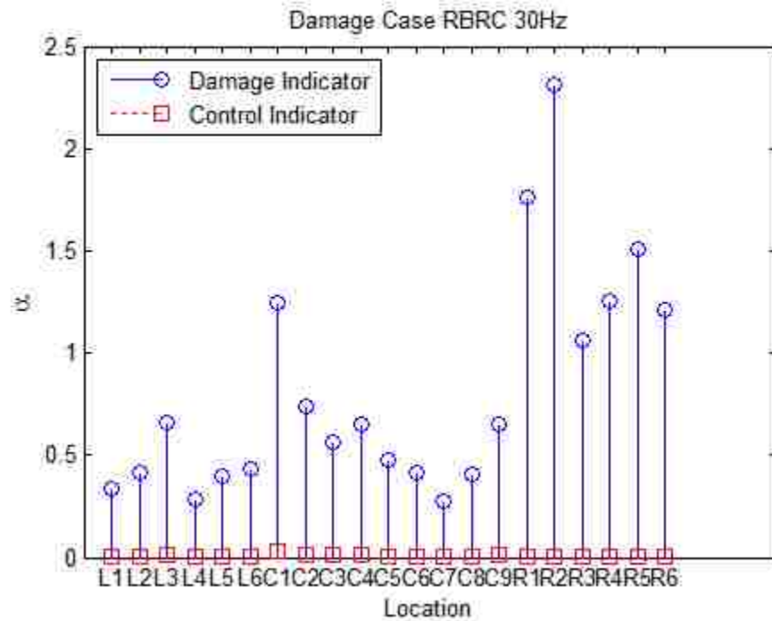
Figure 3.33 Lab Damage Scenario RBRC with 30Hz Input
