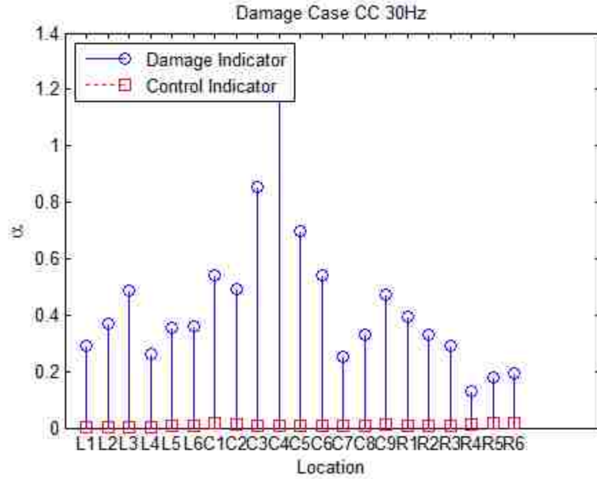
Figure 3.30 Lab Damage Scenario CC with 30Hz Input
