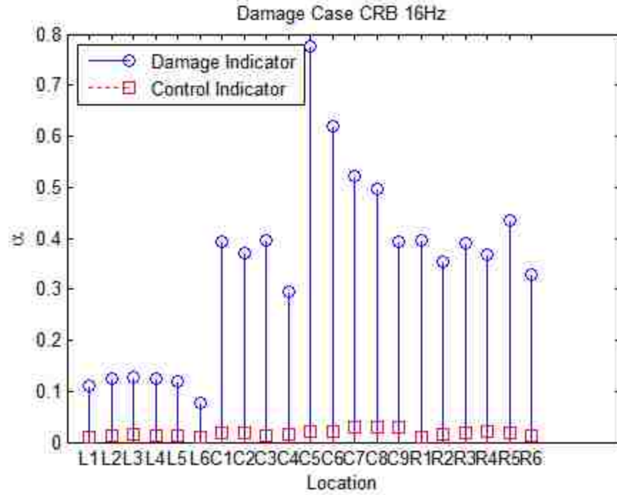
Figure 4.21 Lab Damage Scenario CRB with 16Hz
