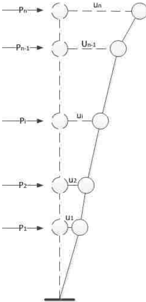
Figure 2.1 Multi-Degree Freedom System
